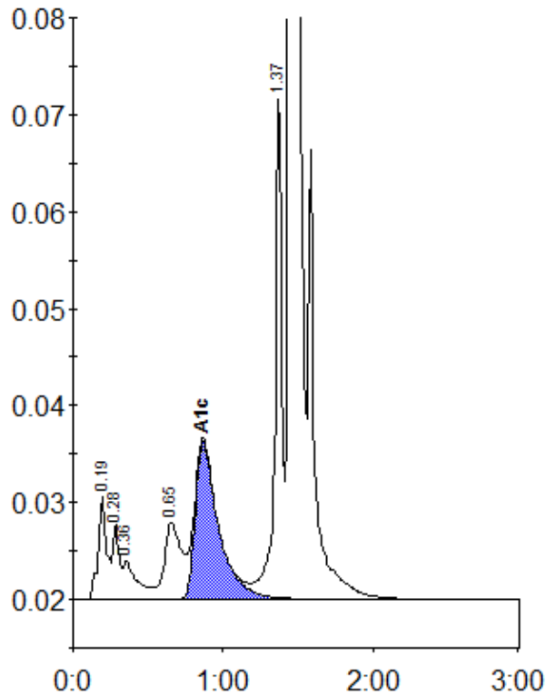
Peak table - ID: 10381399
